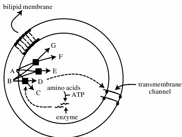
Figure 4. Propagating work and constraint construction in cells. See text for description.
