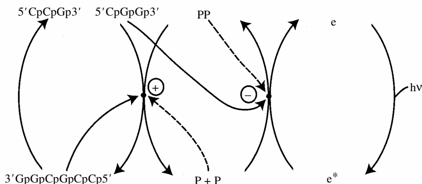
Figure 3. A hypothetical molecular autonomous agent. For clarity, the reaction of the two DNA trimers to form the hexamer without coupling to pyrophosphate breakdown is not shown. See text for description.
