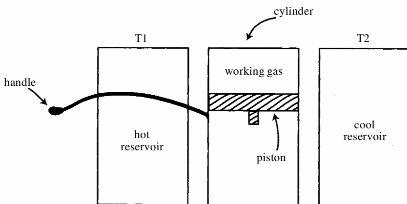
Figure 1. The Carnot cycle with a handle. See text for description.
