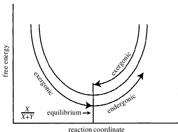
Figure 2. Exergonic and endergonic chemical reactions. See text for description.
